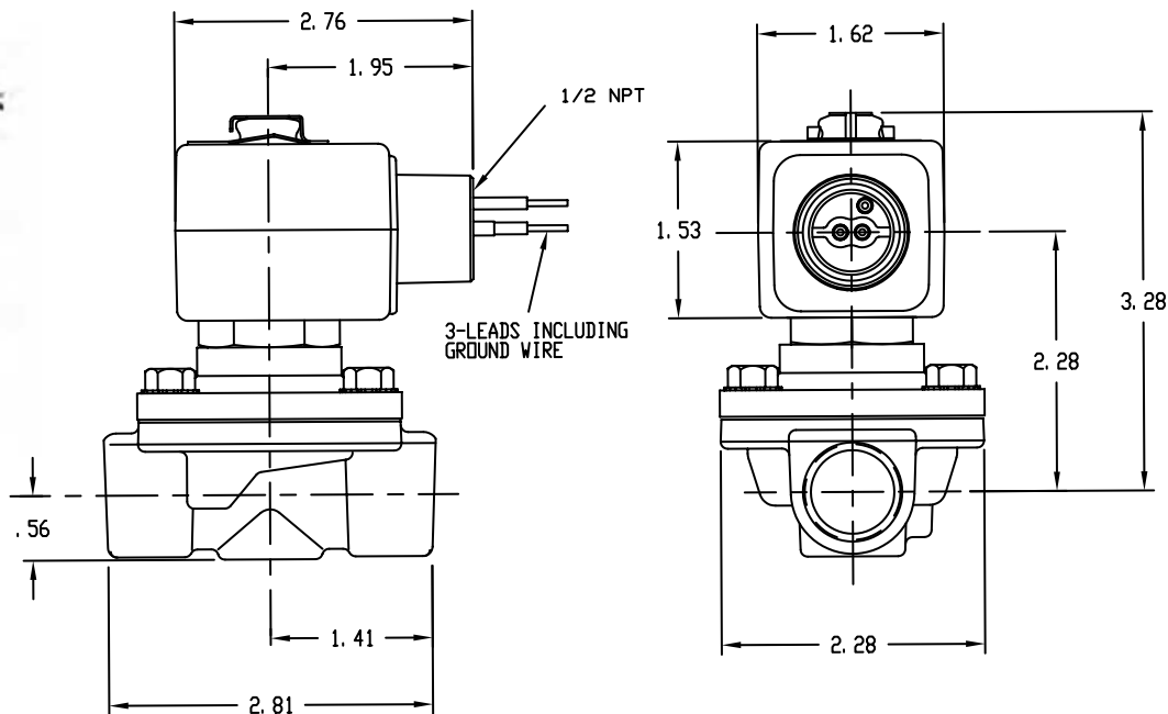
2-Way Normally Open Port Identification: IN-IN/ OUT-OUT
