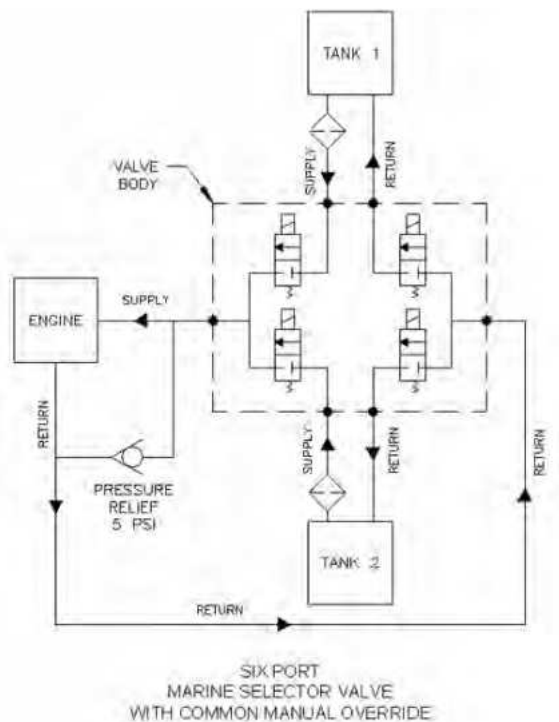
Schematic shows the ease of incorporating the Fuel Selector Manifold into your system
