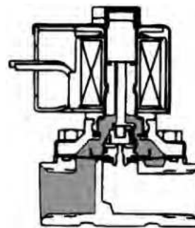
Normally Open, Energized
