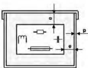
Potting Metallic envelope e > 1 \text{ mm}
