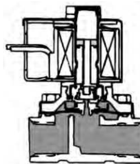
Normally Open, De-Energized
